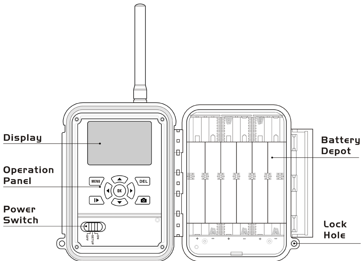
Fig 2 :Operation Interface
